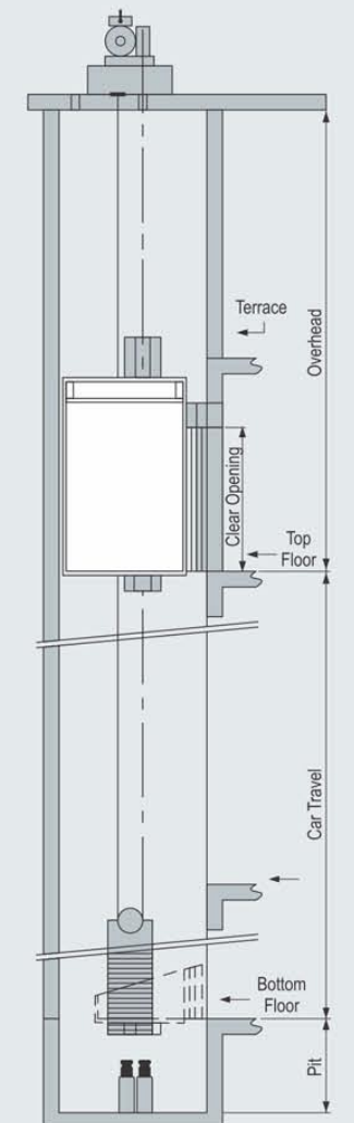
Sectional Elevation of Elevator
