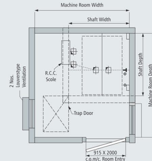
Cross Sectional Machine Room Plan
