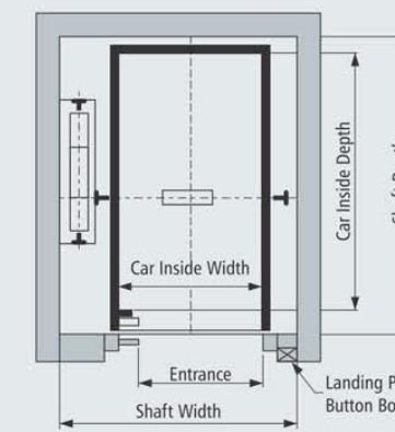
Cross Sectional Lift Shaft Plan Stretcher Lift (manual Door)
